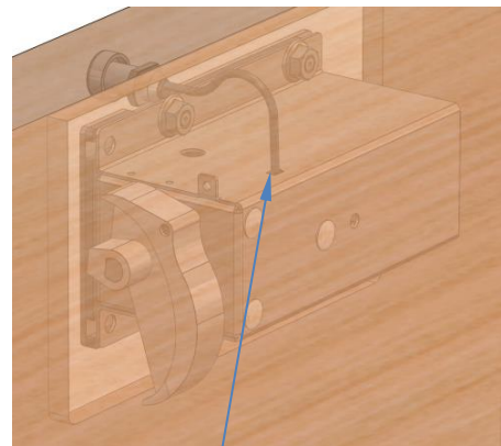
sensor cable
